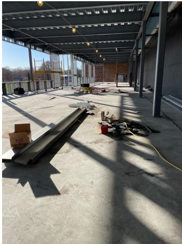
2 nd Floor Slab On Deck
