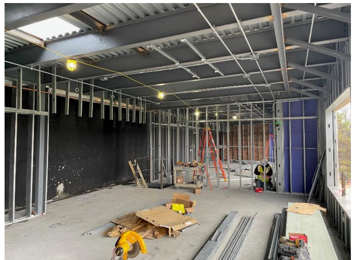
2 nd Floor Interior Framing
