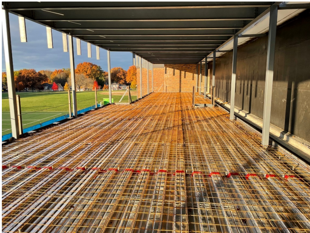
3 rd Floor Metal Deck
