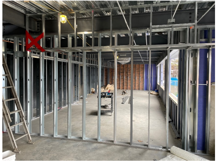
Ground Floor Interior Framing
